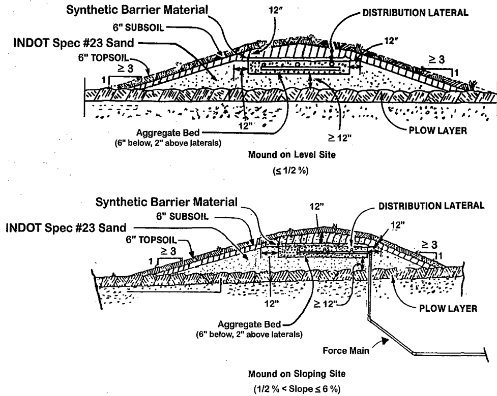
Figure 5 Cross Sections of Elevated Sand Mounds for Level and Sloping Sites
