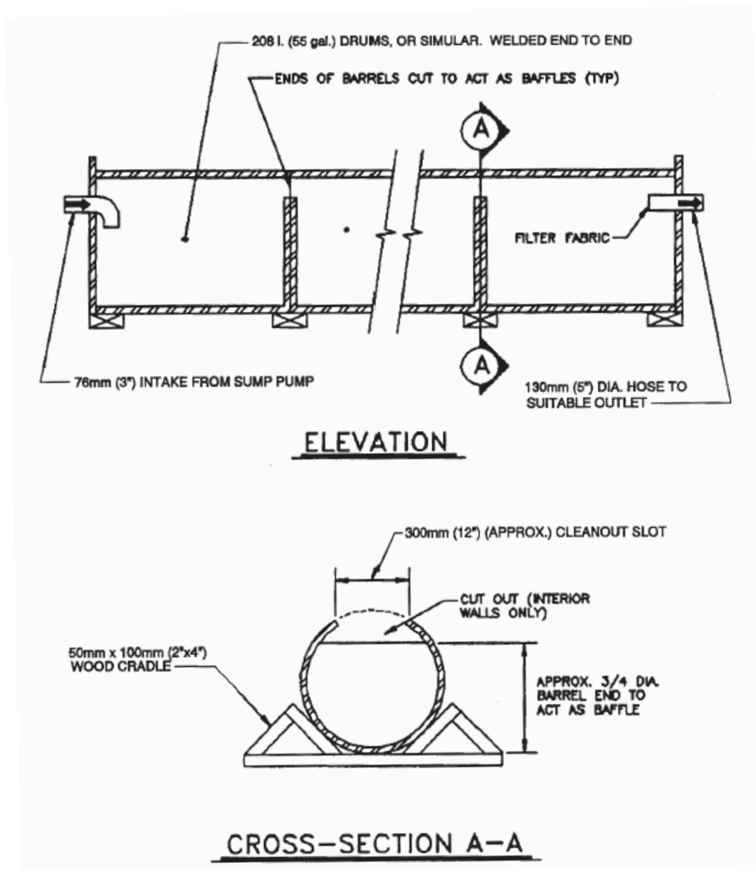
Figure CN-103-A Portable Sediment Tank
