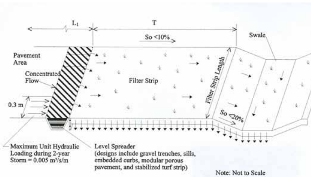
Figure PC-108B Typical Buffer Strip Schematic (SUSMP, 2002)
