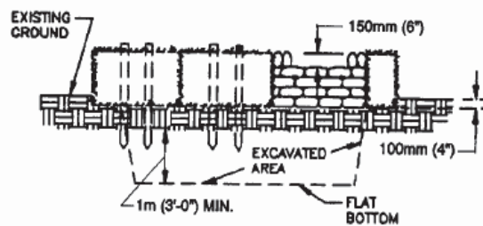
CROSS-SECTION A-A
